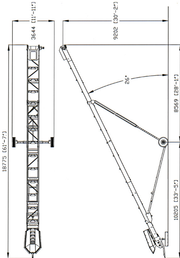
Fig. 2. Discharge Maximum Stockpile height
